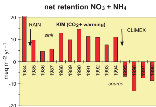
Figure 6: Net catchment fluxes of total N at the CLIMEX experiment in S. Norway. For the 4 years of experimental warming, the catchment became a net source of N rather than a net sink.
