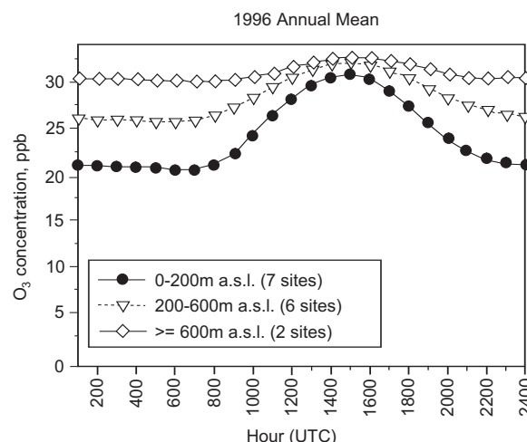
Figure 3: Annual Mean (1996) of the daily cycle of surface ozone concentration at three different altitude categories.
