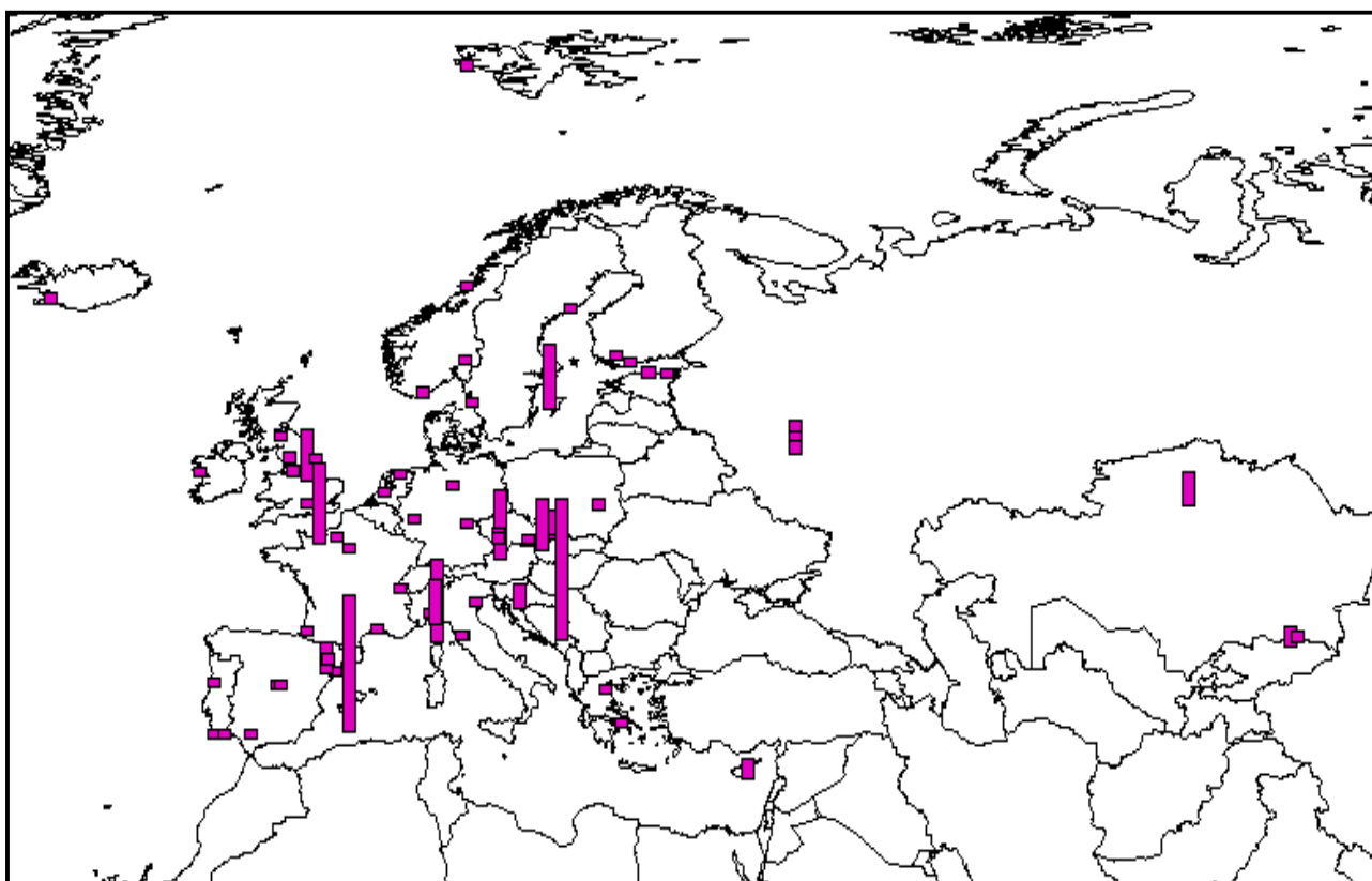
Figure 5b. PCN-29 ('combustion-indicator')
