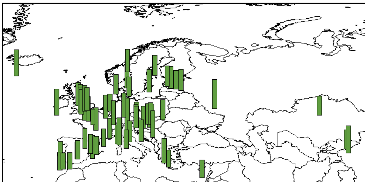
Figure 5 \alpha -HCH and \gamma -HCH
