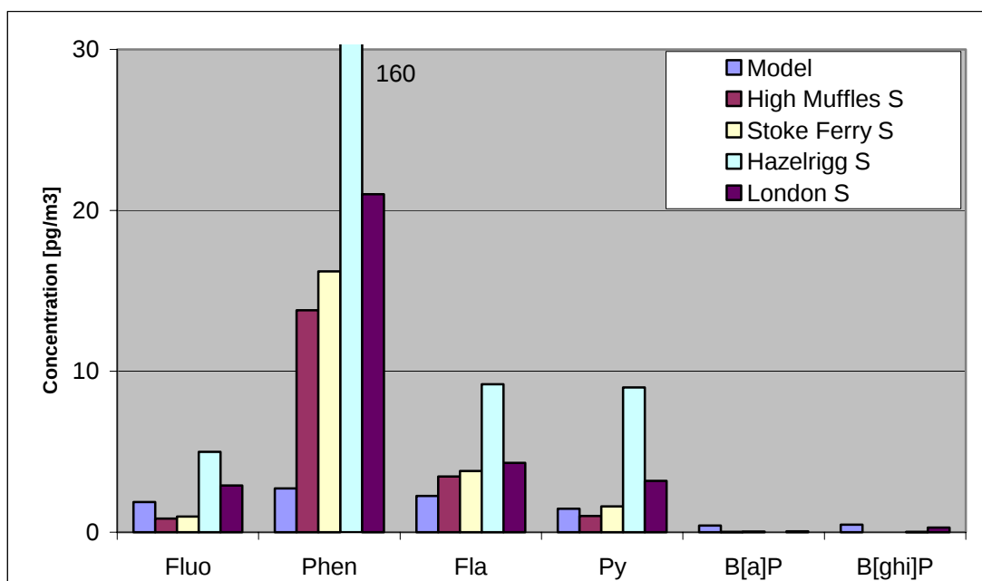
Figure 1a. Summer predicted and measured concentrations
