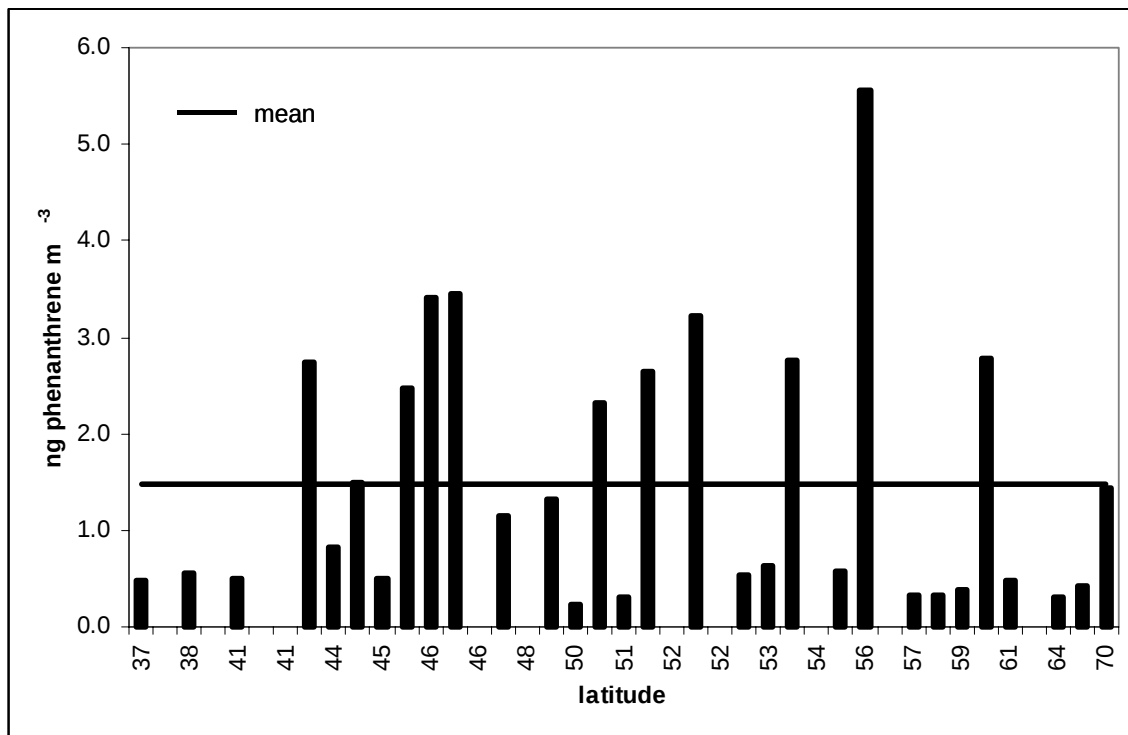
Figure 4. Phenanthrene levels at each site across Europe, showing an average concentration of 1.5 \text{ng m}^{-3} .
