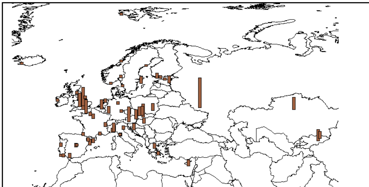
Figure 4. \Sigma_{12}\text{PAH}
