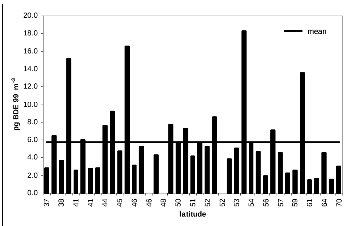
Figure 2. BDE-99 levels at each site across Europe, showing an average concentration of 6 pg m -3 .
