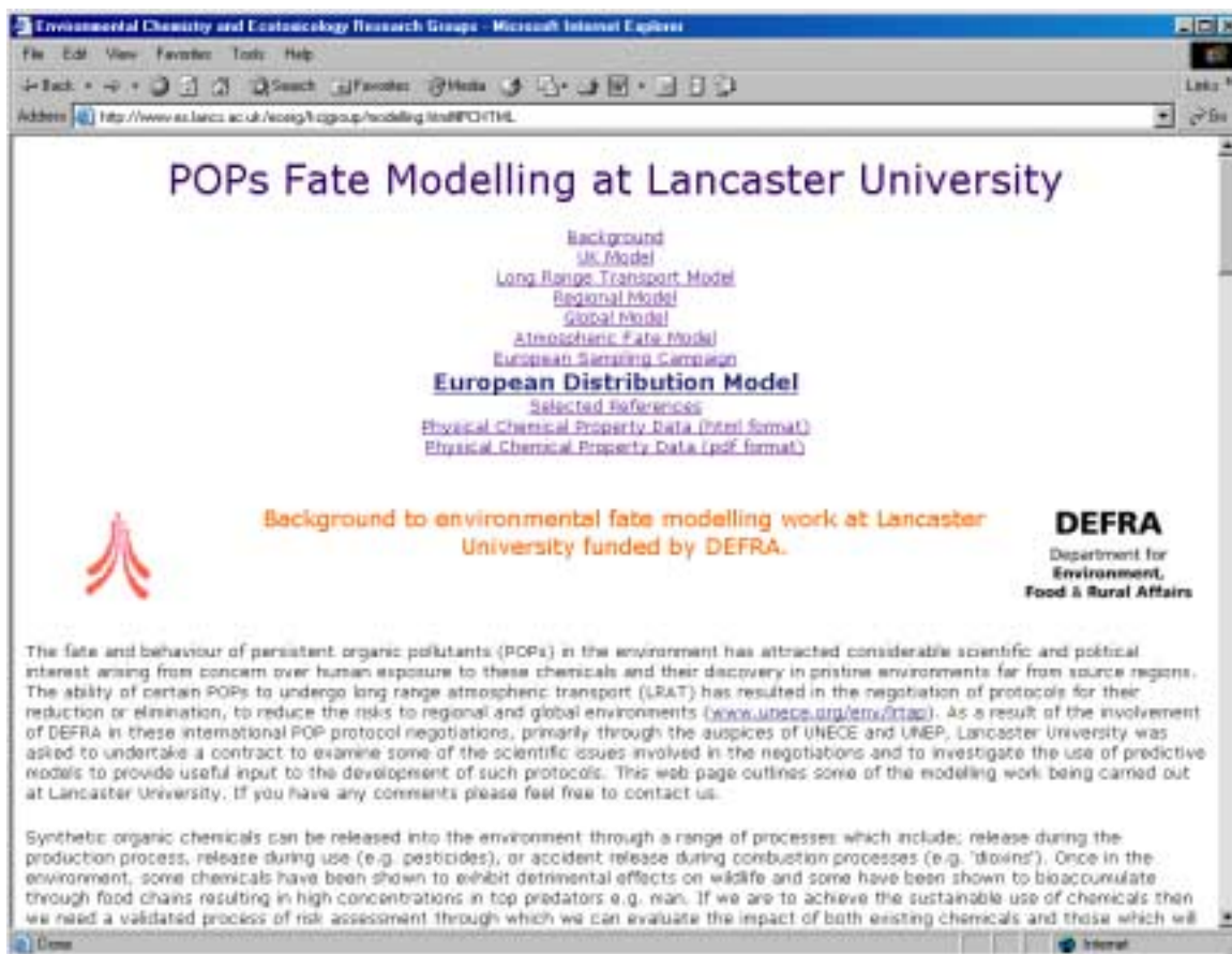
Figure 1 - Web page
