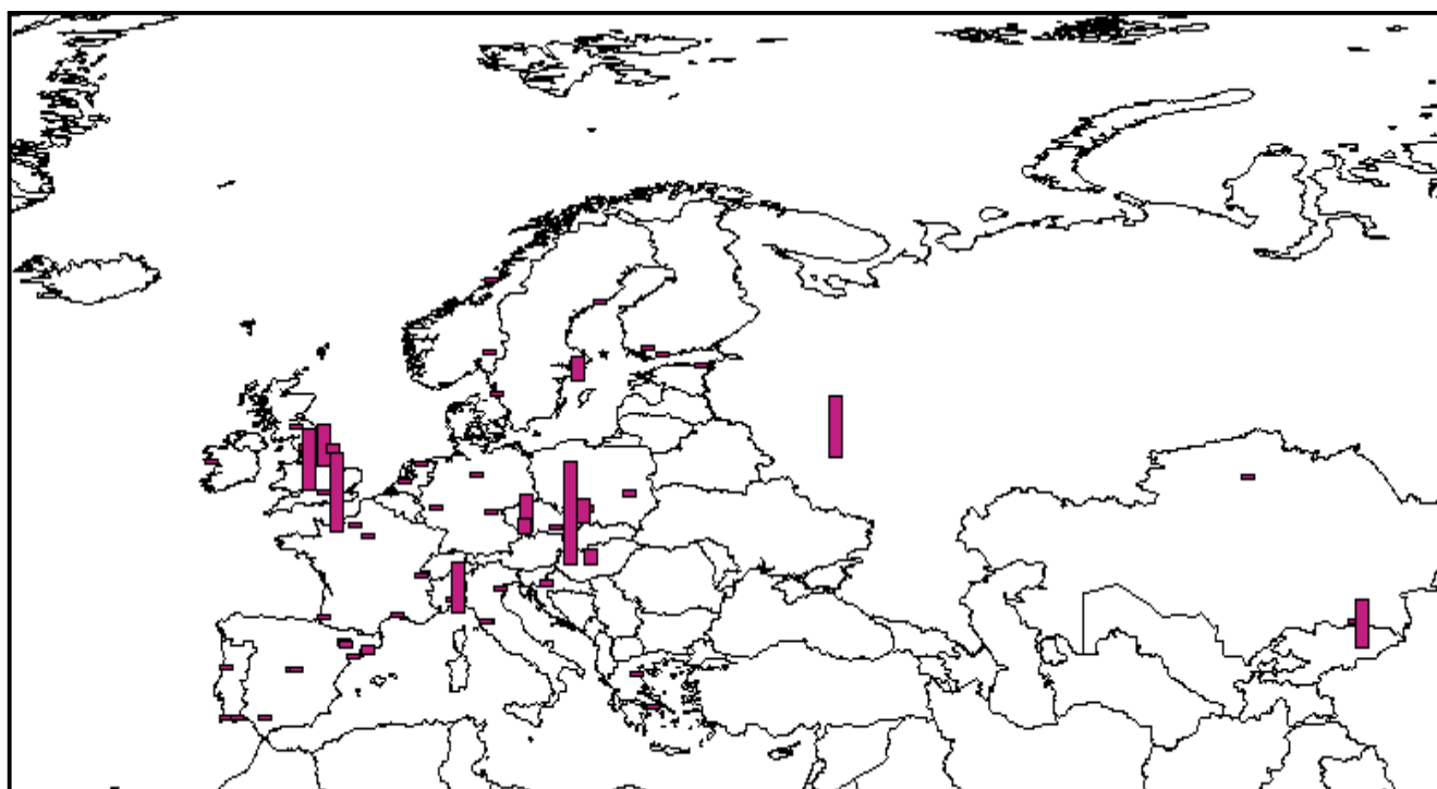
Figure 5a. \Sigma_{11}\text{PCN} (technical-related)
