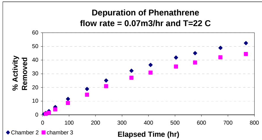
Figure 3 Depuration Rate of ^{14}\text{C} phenanthrene at flow rate of 0.07 \text{ m}^3 \text{ hr}^{-1} and 22^\circ \text{C}
