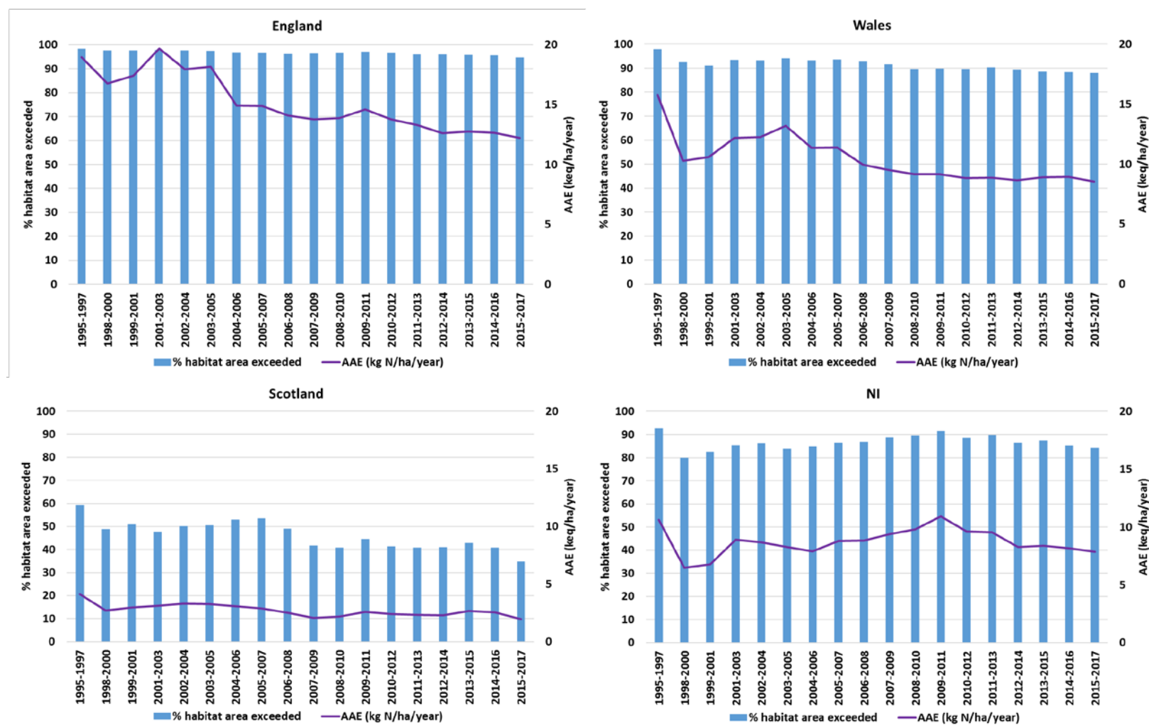
Figure 2.4: Nutrient nitrogen: Percentage area of nitrogen-sensitive habitats with exceedance of nitrogen critical loads, by country and year, and AAE in kg N ha -1 year -1 .
