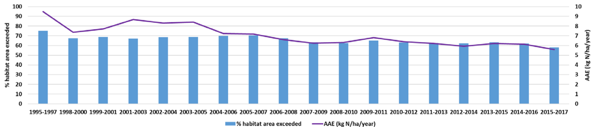
Figure 2.3: Nutrient nitrogen: Percentage area of nitrogen-sensitive habitats with exceedance of nitrogen critical loads in the UK by year, and AAE in kg N ha -1 year -1 .
