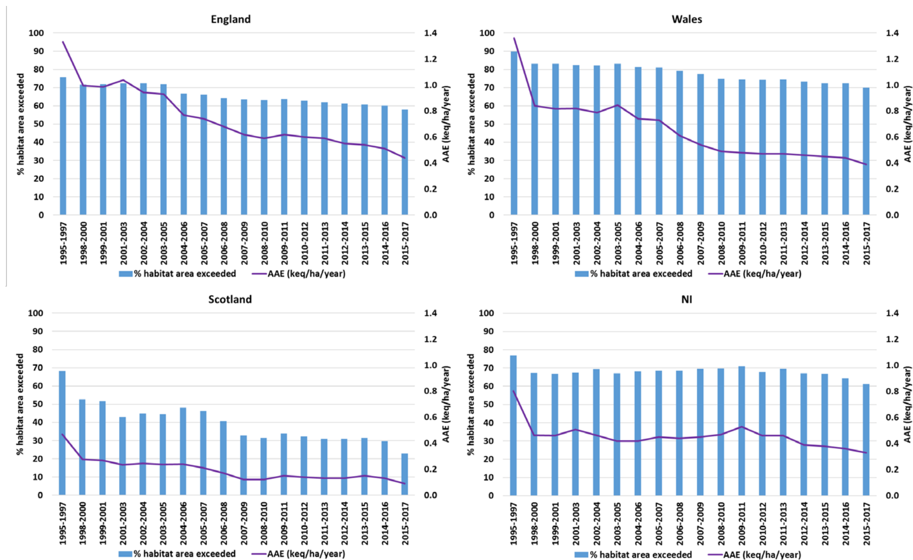
Figure 2.2: Acidity: Percentage area of acid-sensitive habitats with exceedance of acidity critical loads, by country and year, and AAE in keq ha -1 year -1
