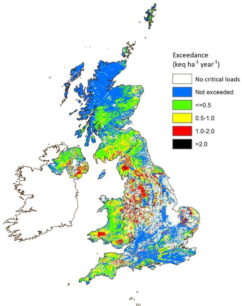
Figure 1.5: Average Accumulated Exceedance (AAE) of critical loads by CBED deposition for 2015-17. Although the legends for the two maps are given in different units, the class intervals are equivalent (i.e. 7 kg N ha -1 year -1 is equivalent to 0.5 keq ha -1 year -1 ).
