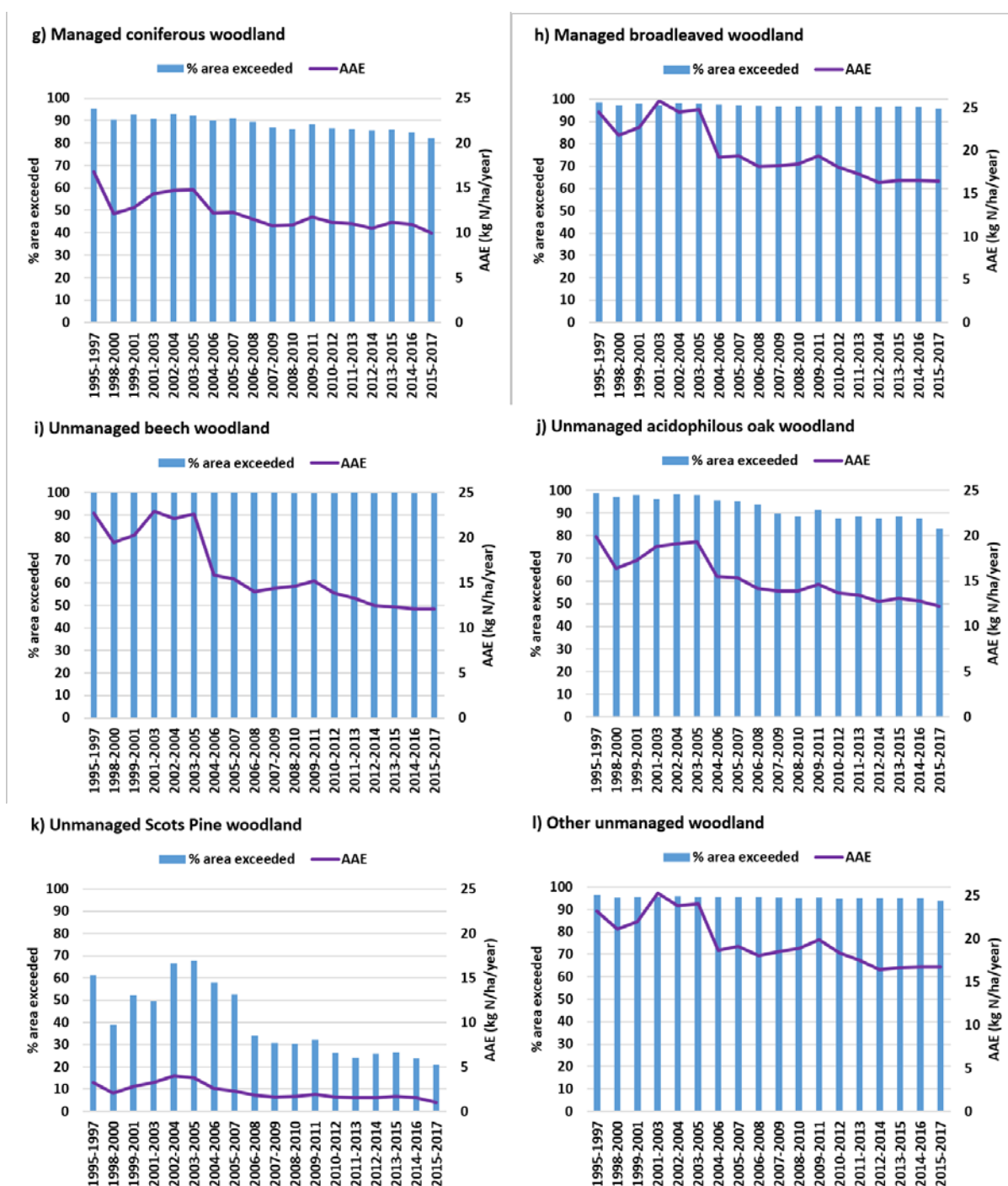
Figure 2.6 (continued): Nutrient nitrogen: Percentage area of habitats where nutrient nitrogen critical loads are exceeded and nutrient nitrogen AAE (in \text{kg N ha}^{-1} \text{ year}^{-1} ) in the UK by deposition dataset year.
