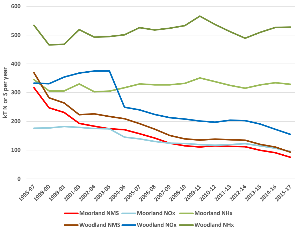
Figure 1.2: Deposition budgets (kilotonnes S or N per year) calculated for all UK 5x5 km grid squares for CBED deposition to moorland and deposition to woodland. NMS = non-marine sulphur, NOx = oxidised nitrogen, NHx = reduced nitrogen.
