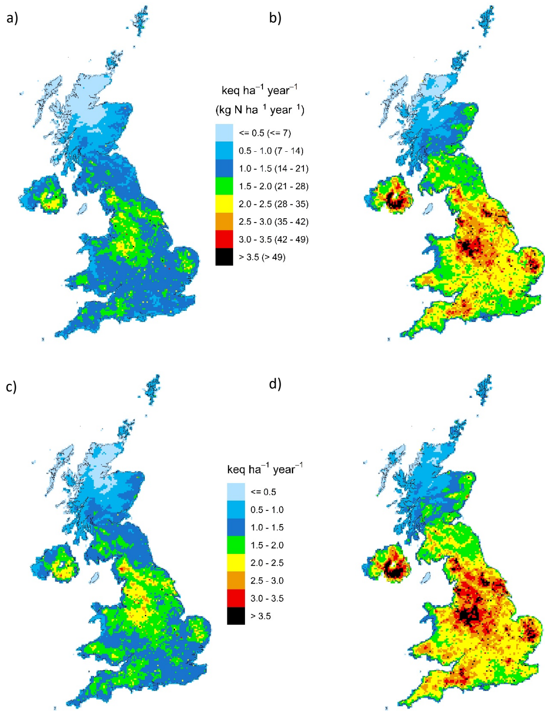
Figure 1.1: CBED deposition for 2015-17: (a) nitrogen (oxidised plus reduced) deposition to moorland; (b) nitrogen (oxidised plus reduced) deposition to woodland; (c) acid (sulphur + nitrogen) deposition to moorland; (d) acid (sulphur + nitrogen) deposition to woodland. Deposition is mapped for N and acidity using the same units (keq ha -1 yr -1 ) and class intervals. For the N maps, deposition rates are also shown in kg N ha -1 yr -1 .
