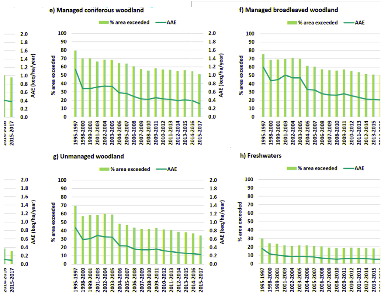
Figure 2.5: Acidity: Percentage area of habitats where acidity critical loads are exceeded, and acidity AAE, for the UK by deposition dataset year.
