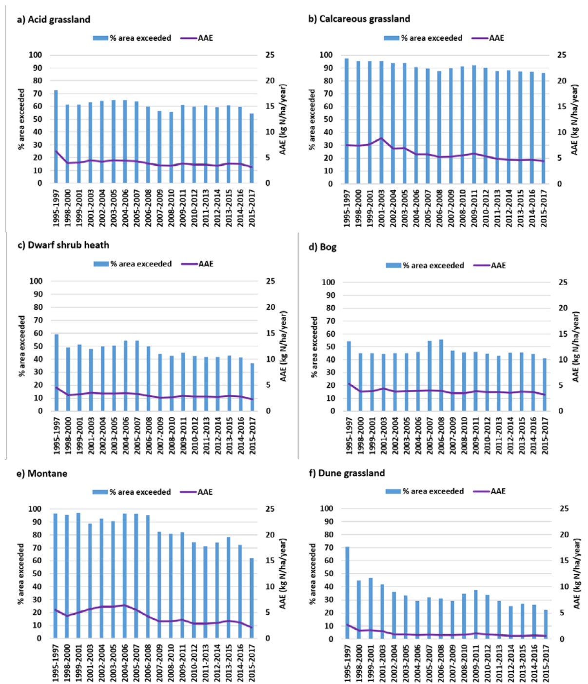
Figure 2.6: Nutrient nitrogen: Percentage area of habitats where nutrient nitrogen critical loads are exceeded and nutrient nitrogen AAE (in kg N ha -1 year -1 ) in the UK by deposition dataset year.
