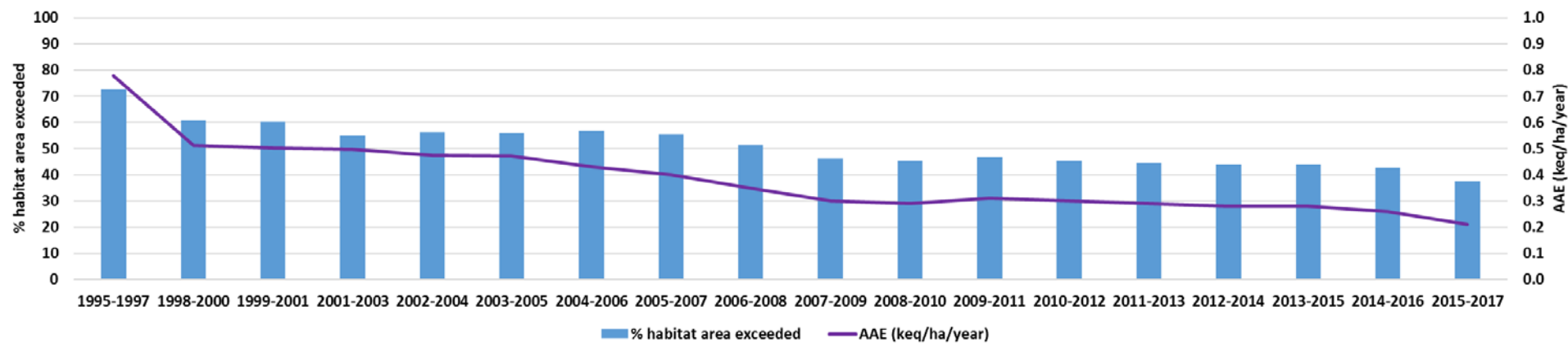
Figure 2.1: Acidity: Percentage area of acid-sensitive habitats with exceedance of acidity critical loads in the UK by year, and AAE in keq ha -1 year -1 .
