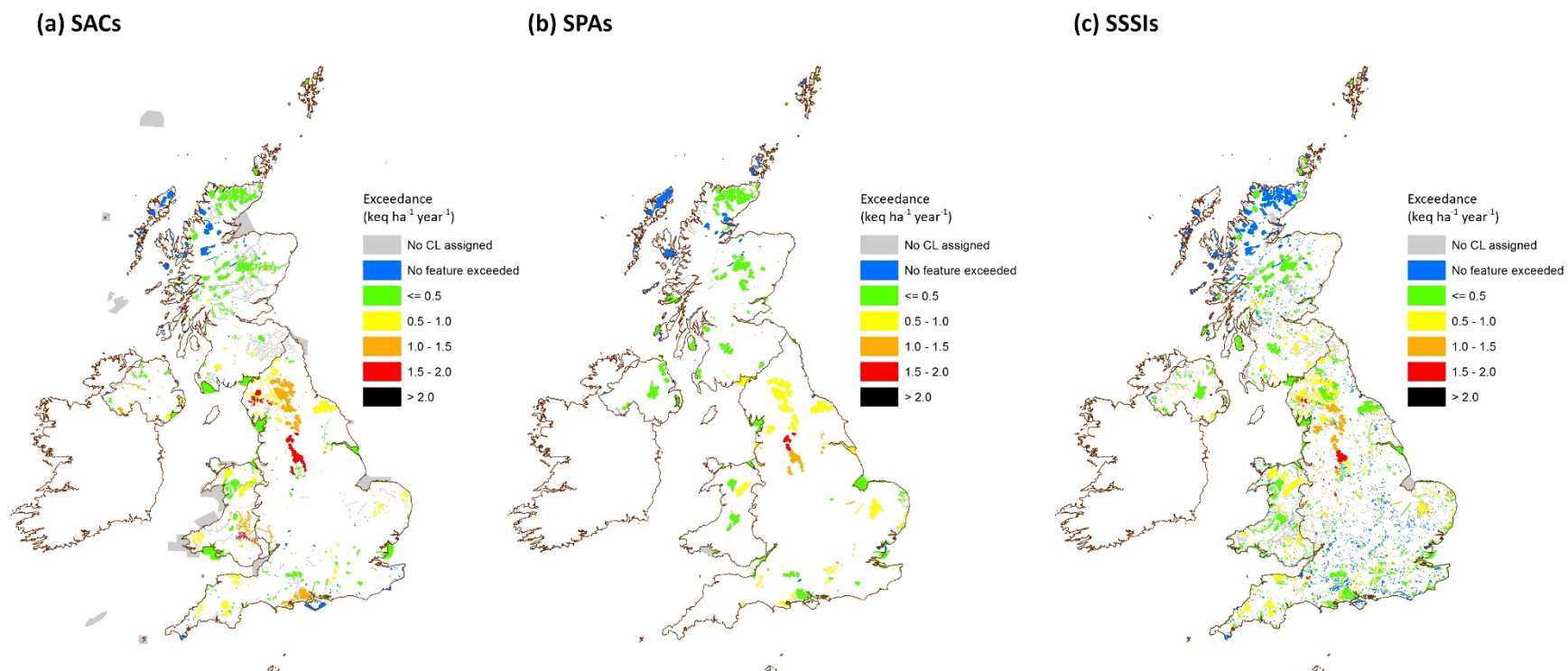
Figure 3.1: Average Accumulated Exceedance (AAE) of acidity critical loads by CBED deposition for 2015-17; maps show the maximum AAE for any feature within each site (other features may have lower or no exceedance).
