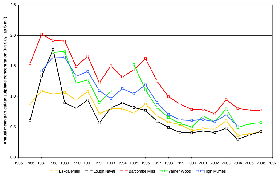
Figure 3-9 Annual mean concentrations of particulate sulphate at the daily sites, from 1986 to 2006 ( \mu\text{g SO}_4^{2-} \text{ as S m}^{-3} )
