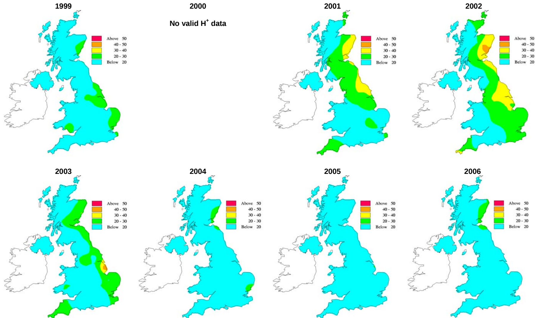
Figure 3-4 Precipitation-weighted concentration maps of Acidity (in \mu\text{eq l}^{-1} ) for 1999-2006
