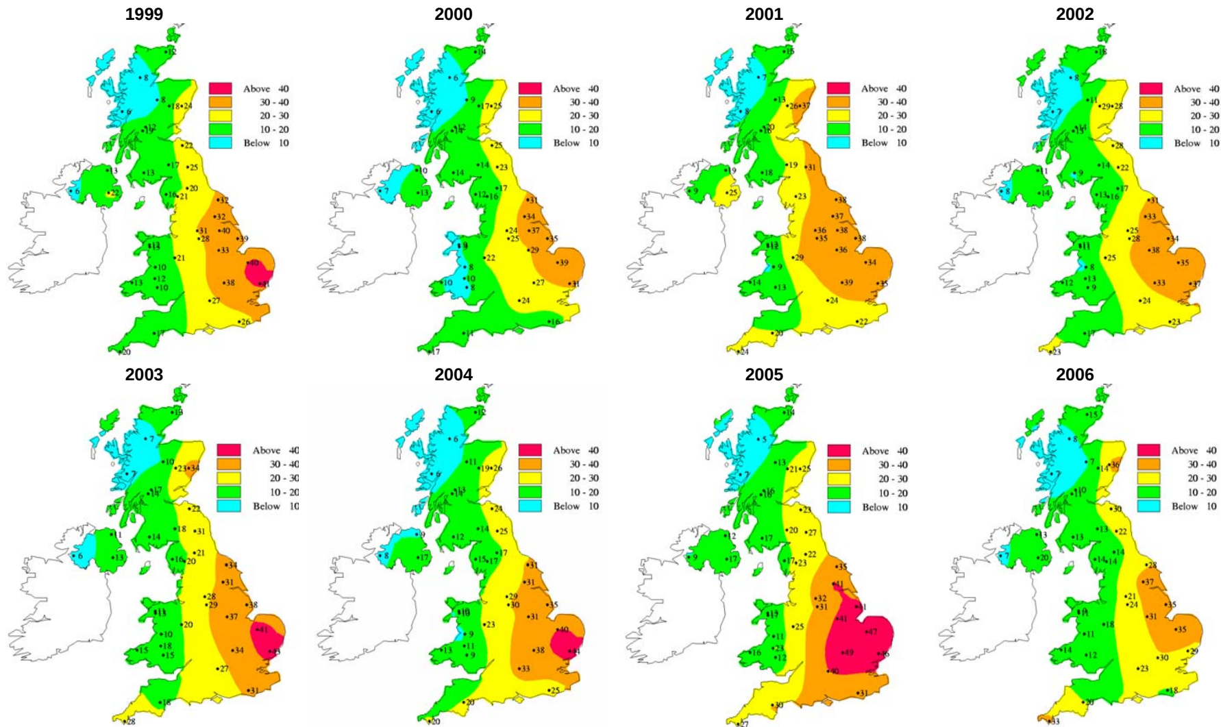
Figure 3-6 Precipitation-weighted Concentration Maps of Nitrate (in \mu\text{eq l}^{-1} ) for 1999-2006
