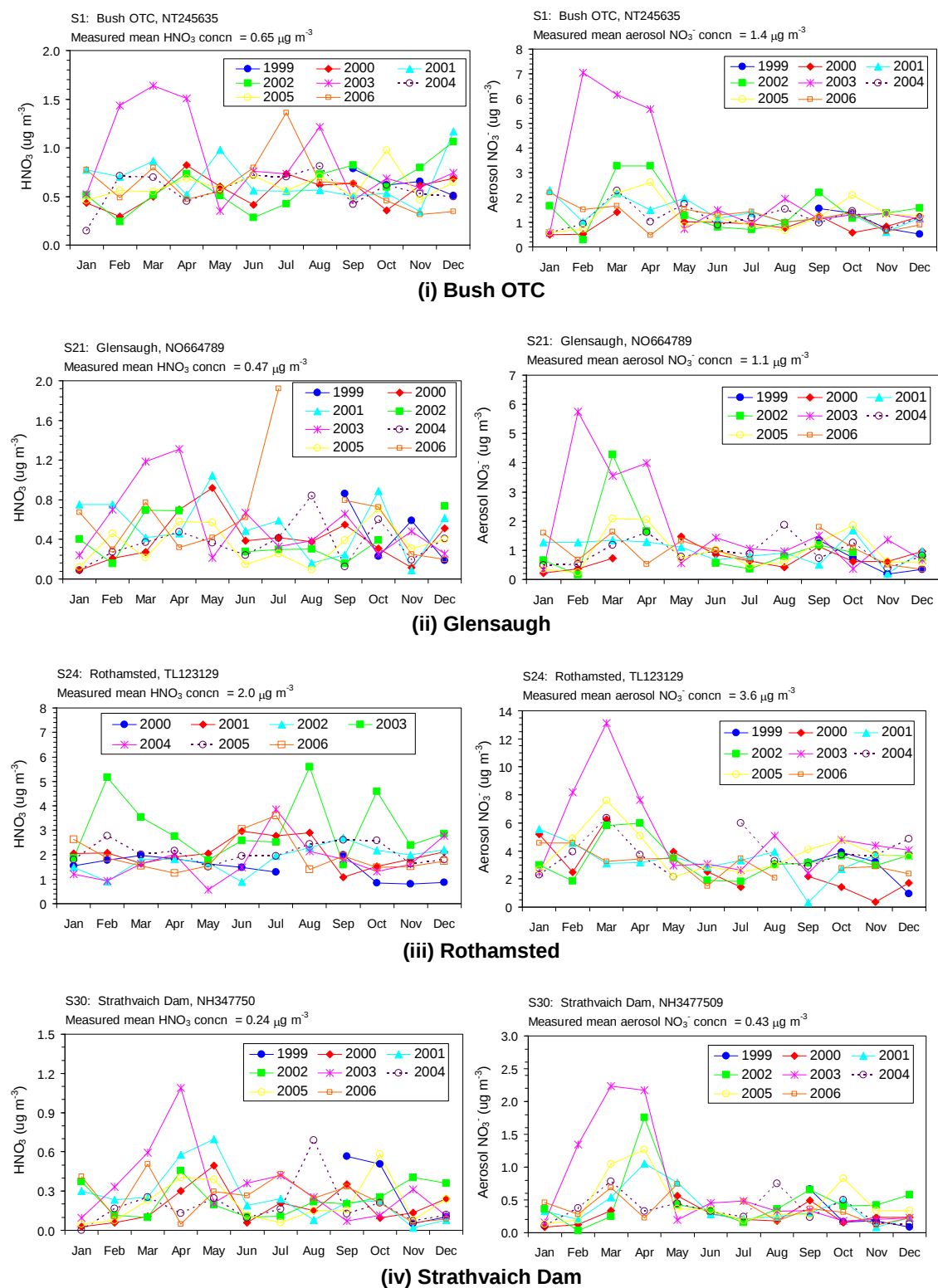
Figure 4-4 Measurements of gaseous \text{HNO}_3 and aerosol \text{NO}_3^- made in the Nitric Acid Monitoring Network between 1999 and 2006
