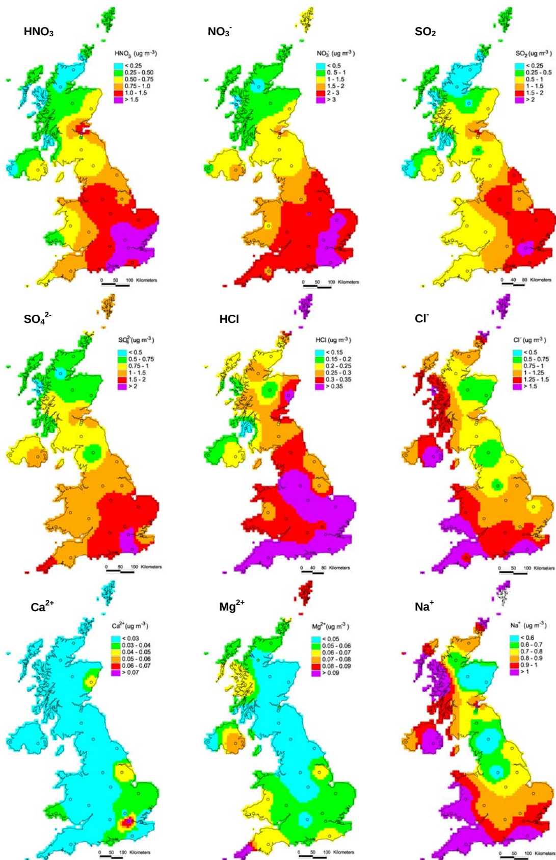
Figure 4-7 Spatial patterns of HNO 3 , SO 2 , HCl and of aerosols NO 3 - , SO 4 2- , Cl - , Ca 2+ , Mg 2+ and Na + concentrations in the UK from averaged monthly measurements made in 2006
