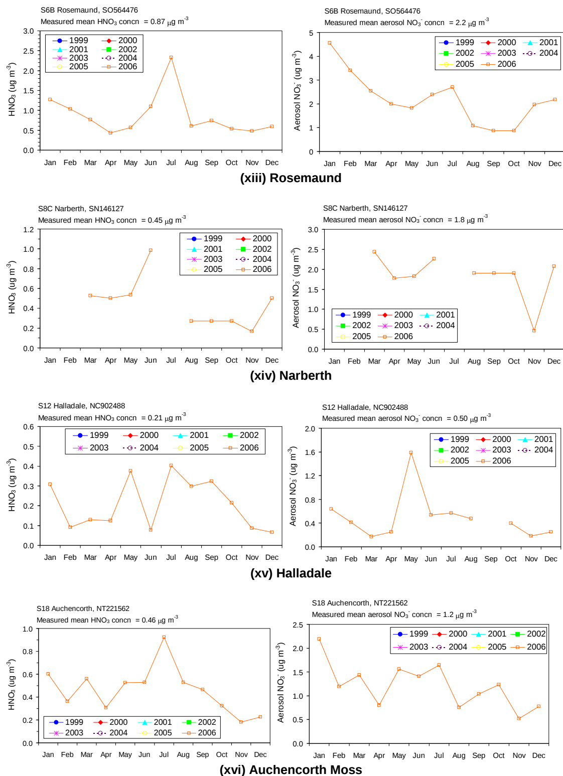
Figure 4-4 Measurements of gaseous \text{HNO}_3 and aerosol \text{NO}_3^- made in the Nitric Acid Monitoring Network between 1999 and 2006 (continued)
