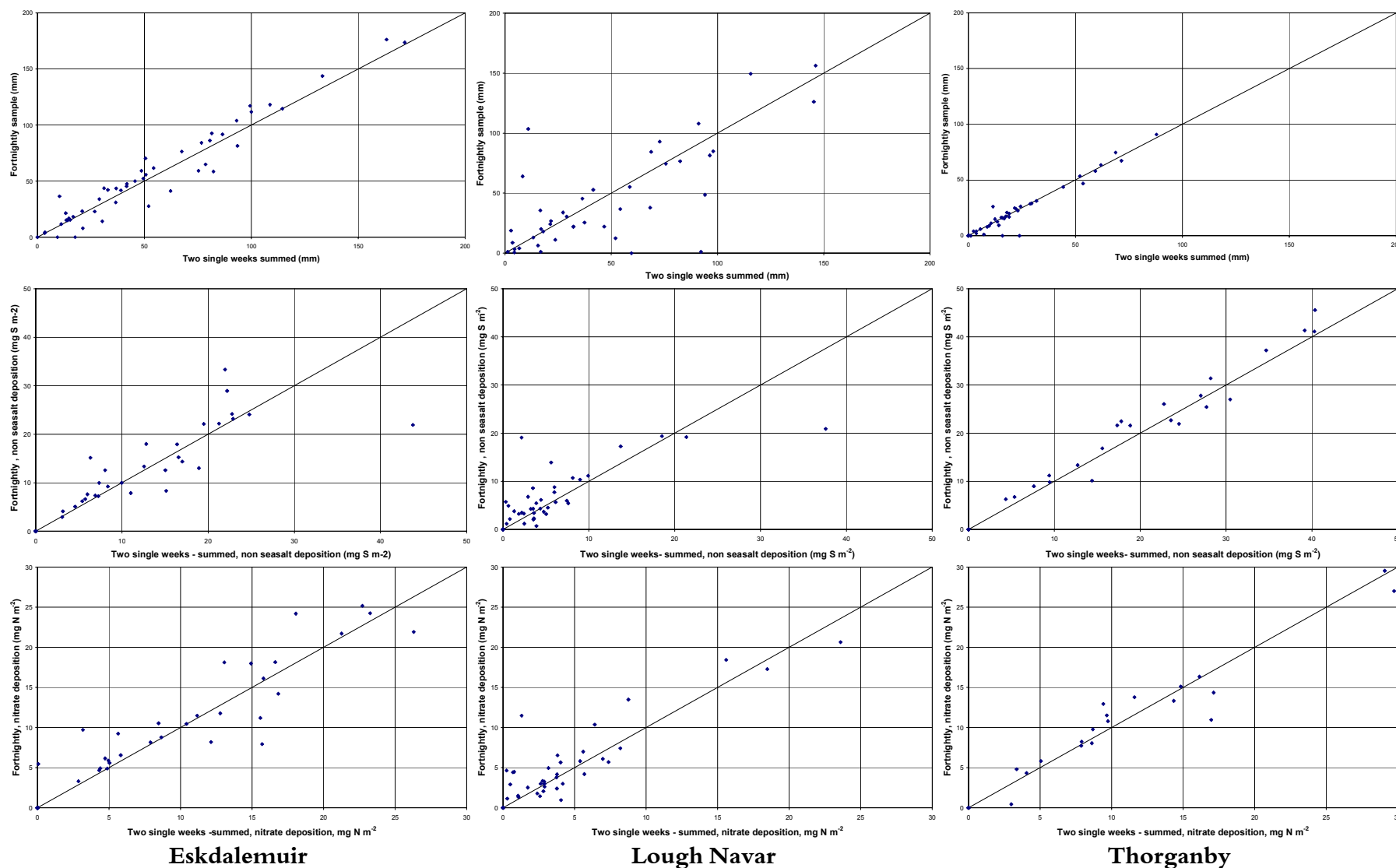
Figure 5.1: A Comparison of Rainwater Volume (top row), Sulphur Deposition (middle row) and Nitrate Deposition (bottom row) measured at Eskdalemuir, Lough Navar and Thorganby.
