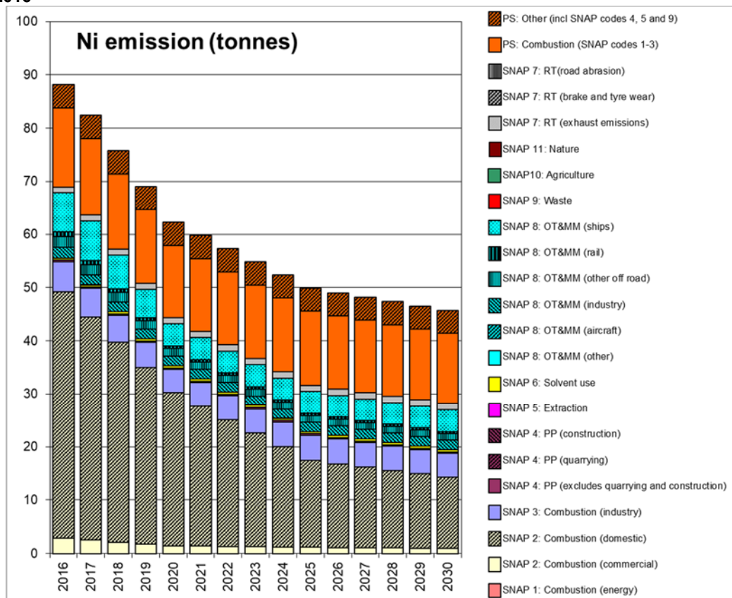
Figure 10-8 - Total UK Ni emissions for 2016 and emissions projections up to 2030 by SNAP code from NAEI 2016
