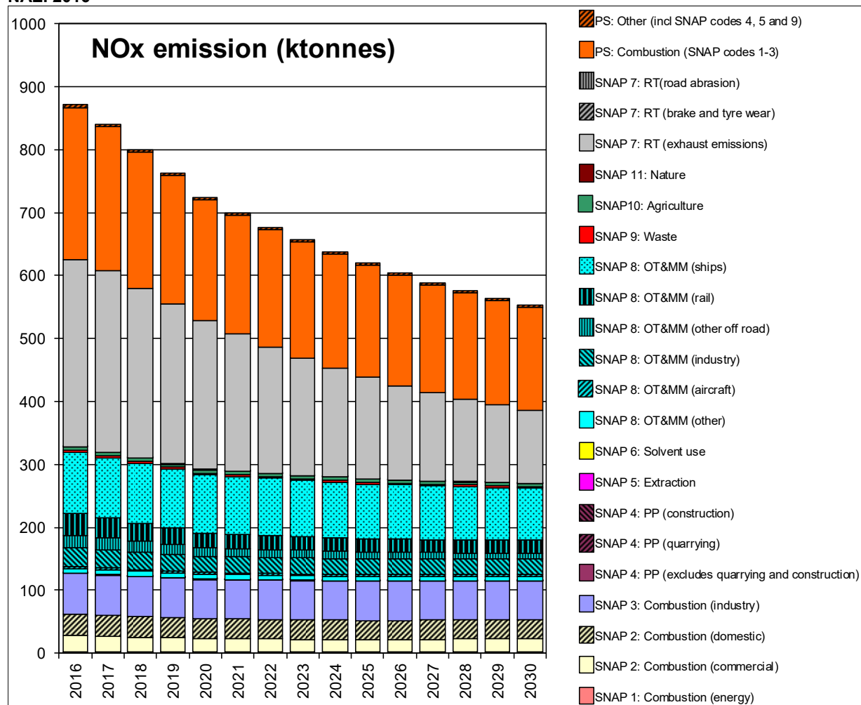
Figure 3-6 - Total UK NO x emissions for 2016 and emissions projections up to 2030 by SNAP code from NAEI 2016
