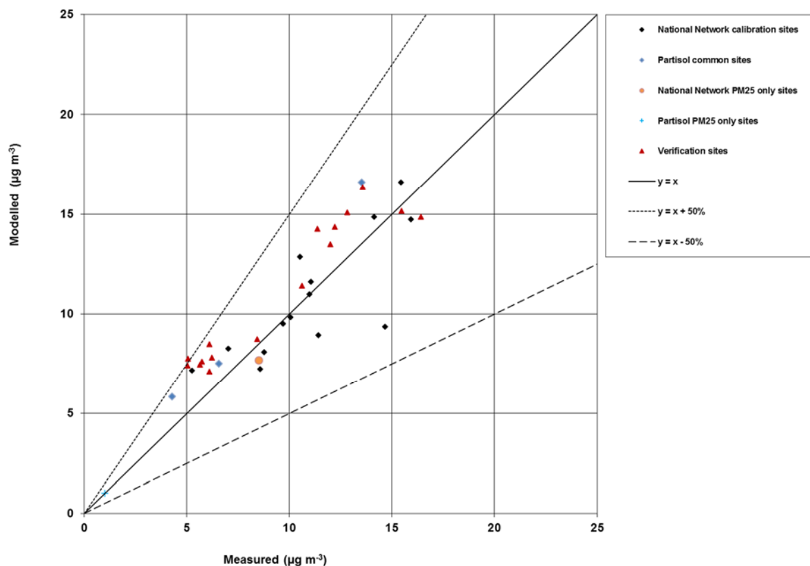
Figure 6-8 - Verification of roadside annual mean PM 2.5 model 2017
