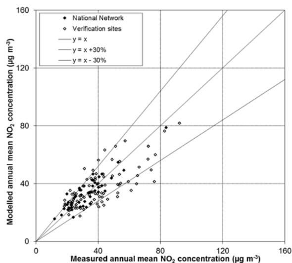
Figure 3-21 - Verification of roadside annual mean \text{NO}_2 model 2017
