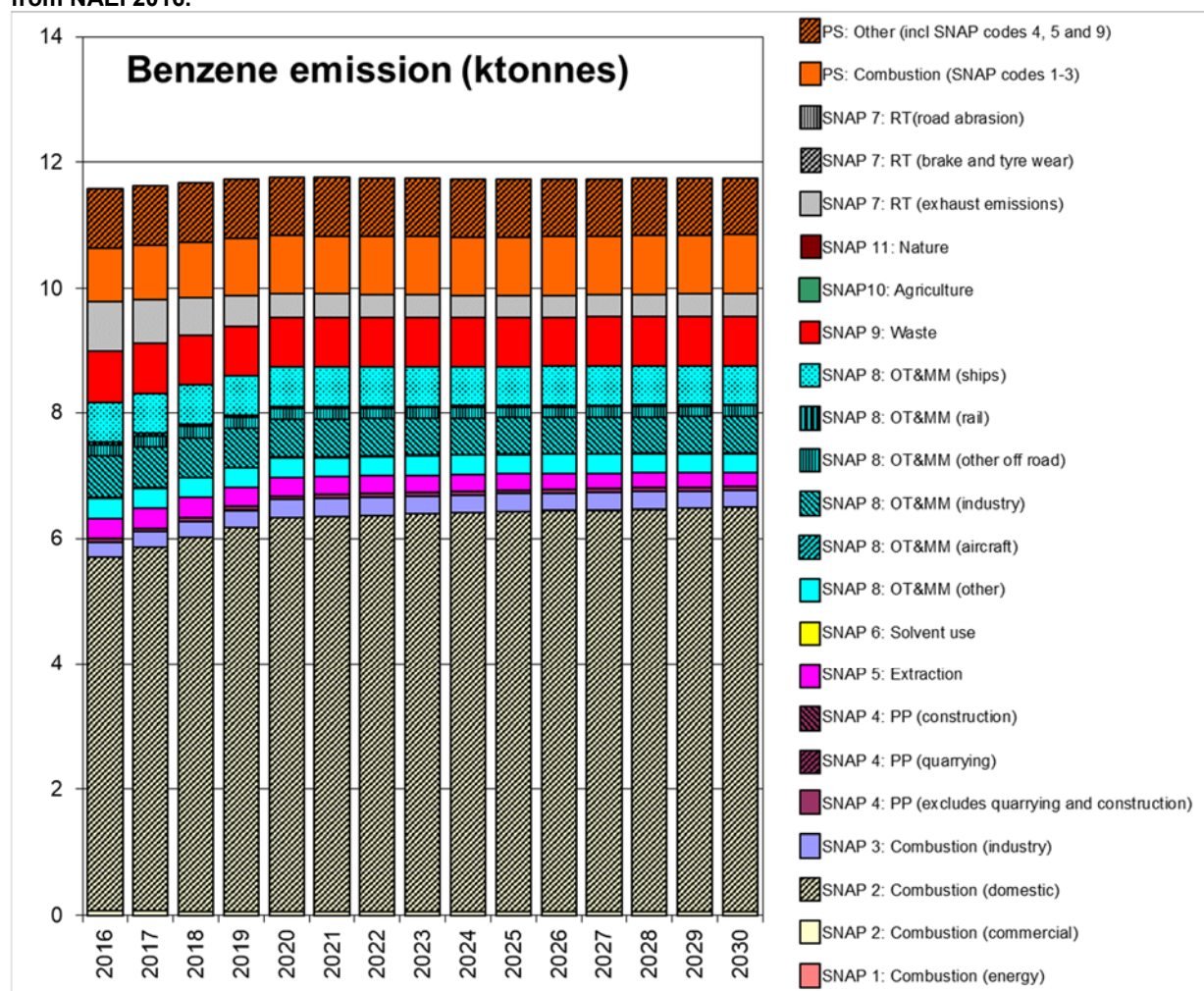
Figure 7-4 - Total UK benzene emissions for 2016 and emissions projections up to 2030 by SNAP code from NAEI 2016.
