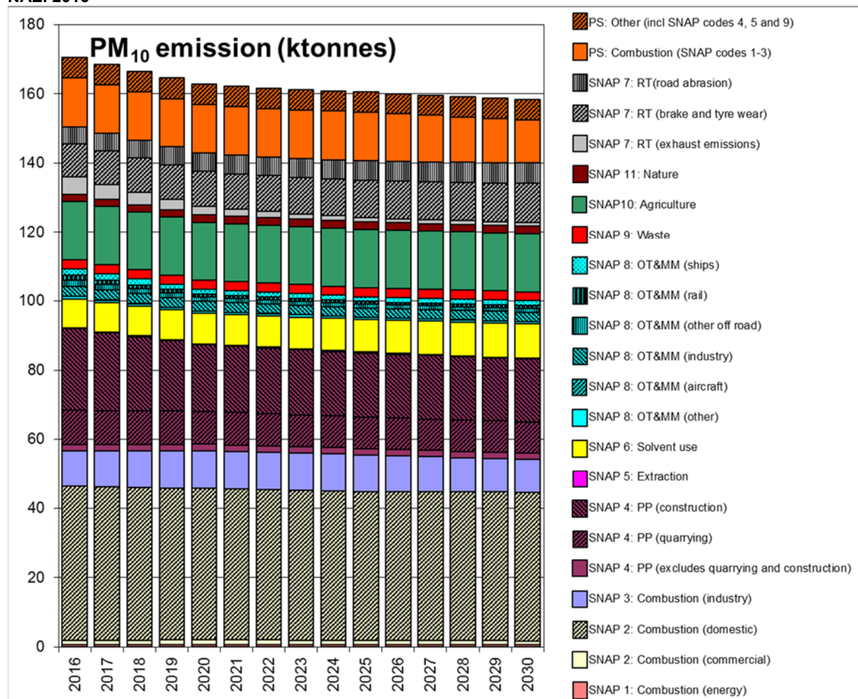
Figure 5-5 - Total UK PM 10 emissions for 2016 and emissions projections up to 2030 by SNAP code from NAEI 2016
