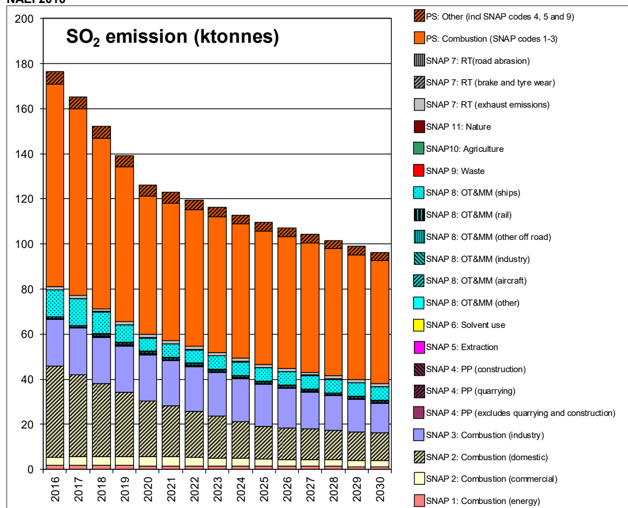
Figure 4-6 - Total UK SO 2 emissions for 2016 and emissions projections up to 2030 by SNAP code from NAEI 2016
