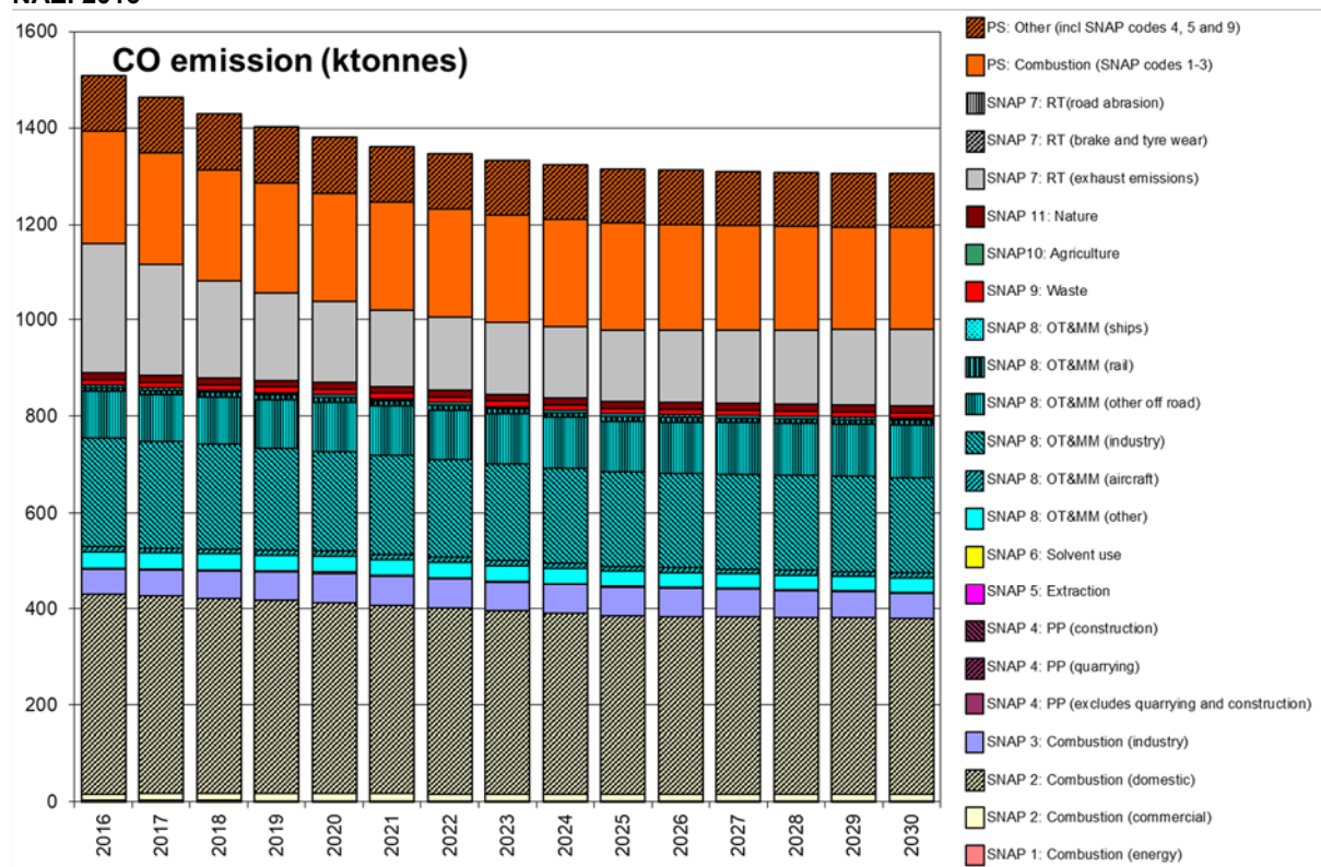
Figure 8-1 - Total UK CO emissions for 2016 and emissions projections up to 2030 by SNAP code from NAEI 2016
