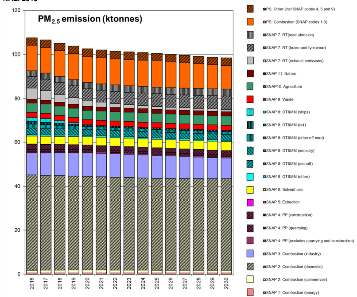
Figure 6-4 - Total UK PM 2.5 emissions for 2016 and emissions projections up to 2030 by SNAP code from NAEI 2016
