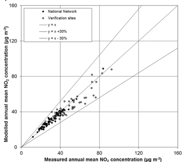
Figure 3-15 - Verification of roadside relationship at roadside locations in 2017
