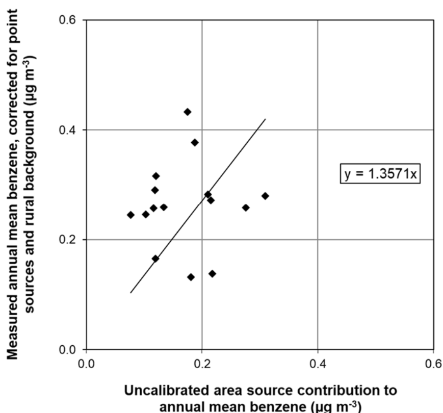
Figure 7-5 - Calibration of area source benzene model, 2017 ( \mu\text{g m}^{-3} )
