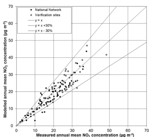
Figure 3-21 - Verification of roadside annual mean \text{NO}_2 model 2017
