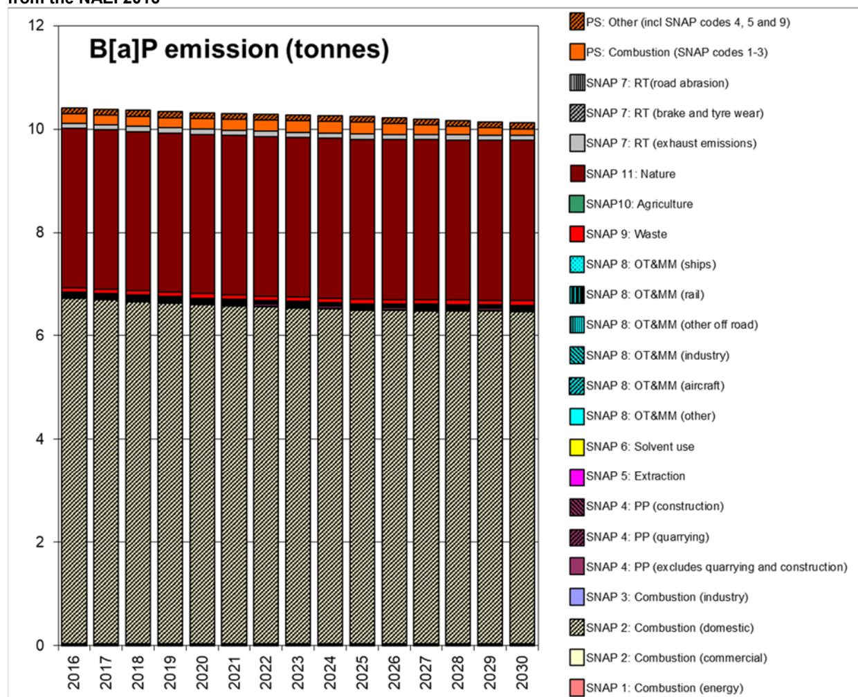
Figure 11-3 – Total UK B(a)P emissions for 2016 and emissions projections up to 2030 by SNAP code from the NAEI 2016
