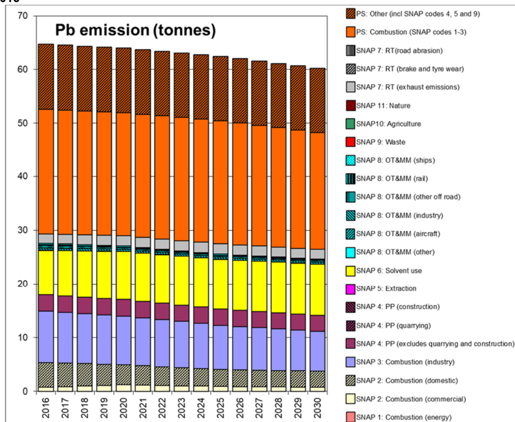
Figure 10-9 - Total UK Pb emissions for 2016 and emissions projections up to 2030 by SNAP code from NAEI 2016
