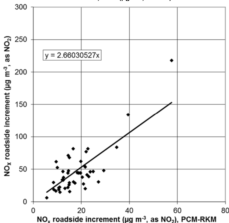
Figure 3-9 - Calibration of \text{NO}_x PCM RKM model, 2017 ( \mu\text{g m}^{-3} , as \text{NO}_2 )
