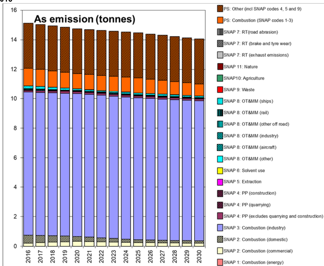
Figure 10-6 - Total UK As emissions for 2016 and emissions projections up to 2030 by SNAP code from NAEI 2016
