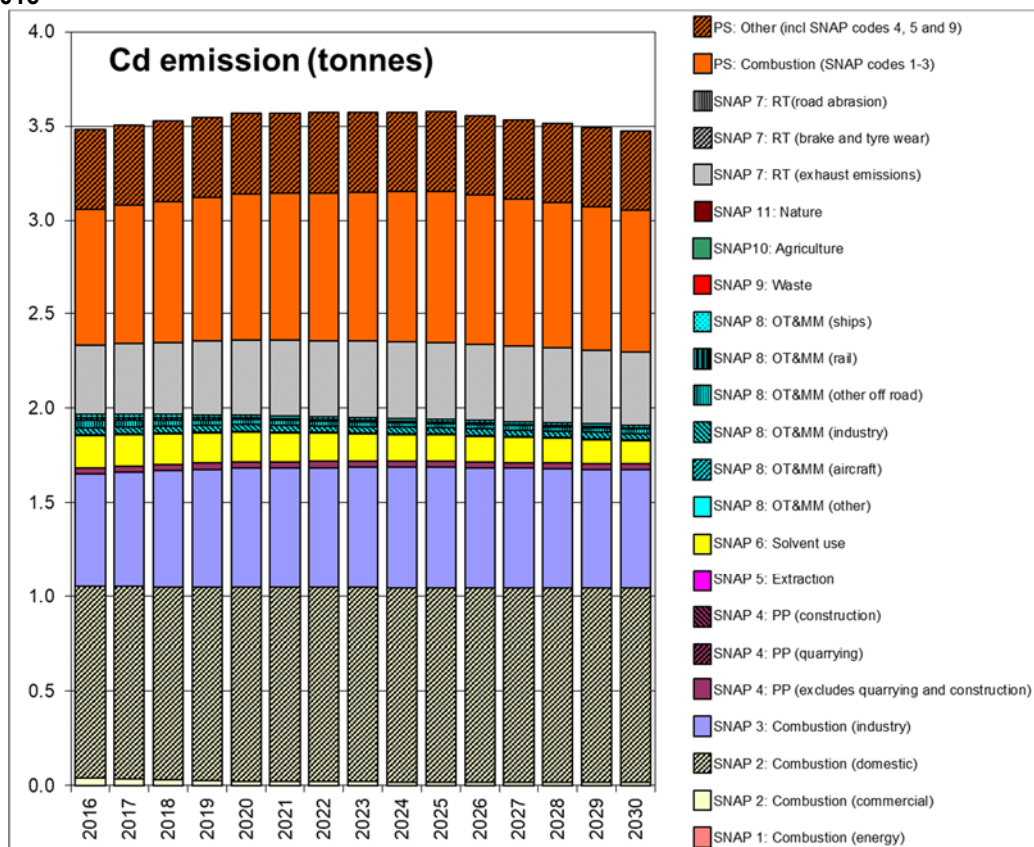
Figure 10-7 - Total UK Cd emissions for 2016 and emissions projections up to 2030 by SNAP code from NAEI 2016
