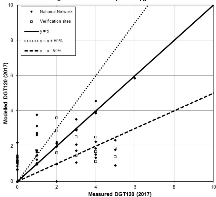
Figure 9-6 - Verification of background number of days > 120 \mu\text{g m}^{-3} model 2017
